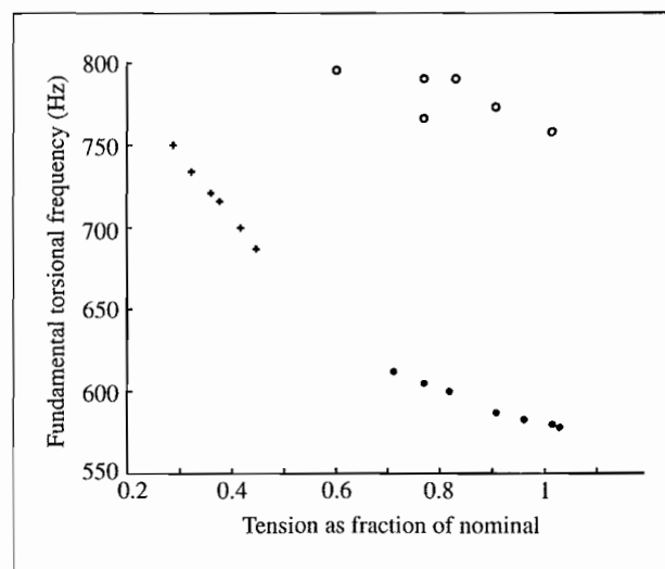
Figure 2. Best-fitted fundamental torsional frequency as a function of string tension. Open circles: nylon-cored string; solid circles: steel-cored string; crosses: gut-cored string.
